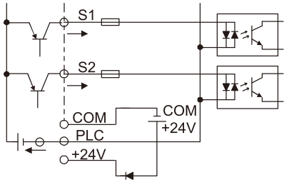
External power supply (PNP mode)
